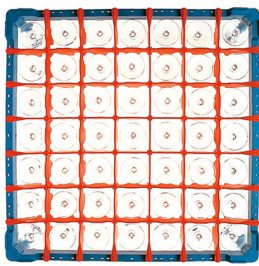
921549 RACK FOR GLASSES SQUARE COMPARTMENT 7 x 7 h. 215
