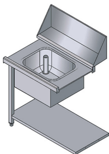
WMV80DX ENTRY TABLE WITH SINK RIGHT-HAND SIDE
