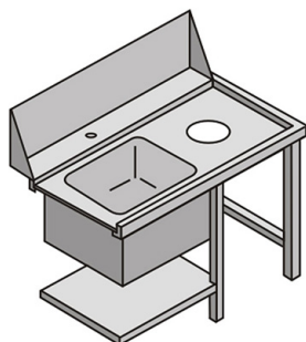
TVSDX TABLE WITH SINK AND WASTING HOLE RIGHT-HAND SIDE ENTRY
