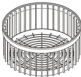
5782A ROUND BASKET ø380 x 170 mm
