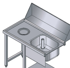
PVSX TABLE WITH SINK - LEFT- HAND SIDE ENTRY FOR MODELS ATR1500 AND ATR1800
