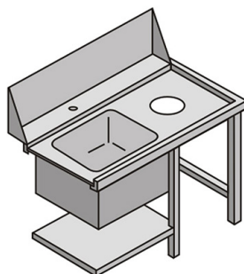
TVSFX TABLE WITH SINK AND WASTING HOLE FRONTAL ENTRY
