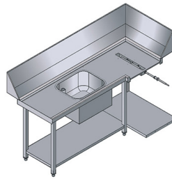
WTM90DX MECHANIZED TABLE ENTRY 90° RIGHT-HAND SIDE WITH SINK
