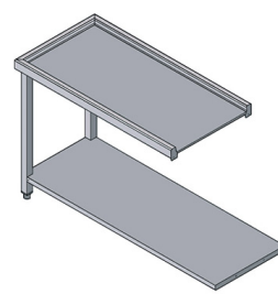
WT100E ENTRY TABLE
