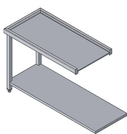
P110E ENTRY TABLE FOR MODELS ATR1500 AND ATR1800
