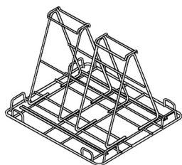
14284 RACK FOR 4 TRAYS 1/1 GN
