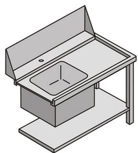
TVDX TABLE WITH SINK RIGHT- HAND SIDE ENTRY
