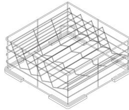
7186 BASKET FOR GLASSES 400 x 400 x 180 mm
