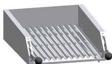
K7GRC05M LAVASTONE GRILLS - MOVABLE STEEL GRATE FOR MEAT 1/2 MODULE
